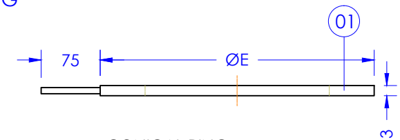
CONICAL RING
