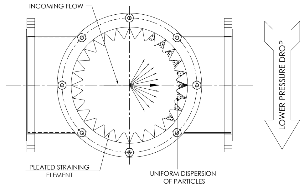
TOP VIEW - BASKET STRAINER - PLEATED STRAINING ELEMENT
