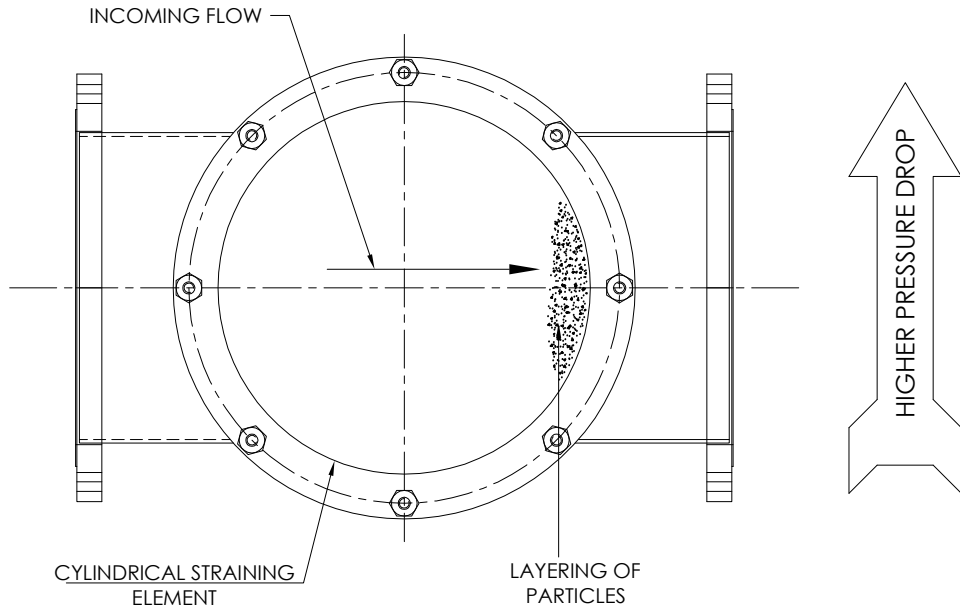
TOP VIEW - BASKET STRAINER - CYLINDRICAL STRAINING ELEMENT
