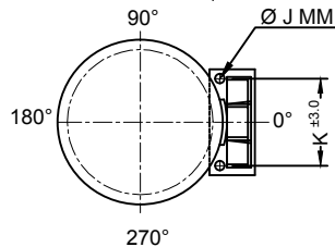
FOUNDATION DETAIL
